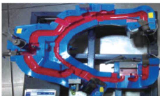
▲ HOSE ASSY
