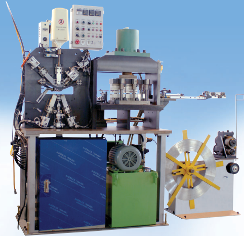
▲ CLAMP SEAL RETAINING AUTO' M/C
